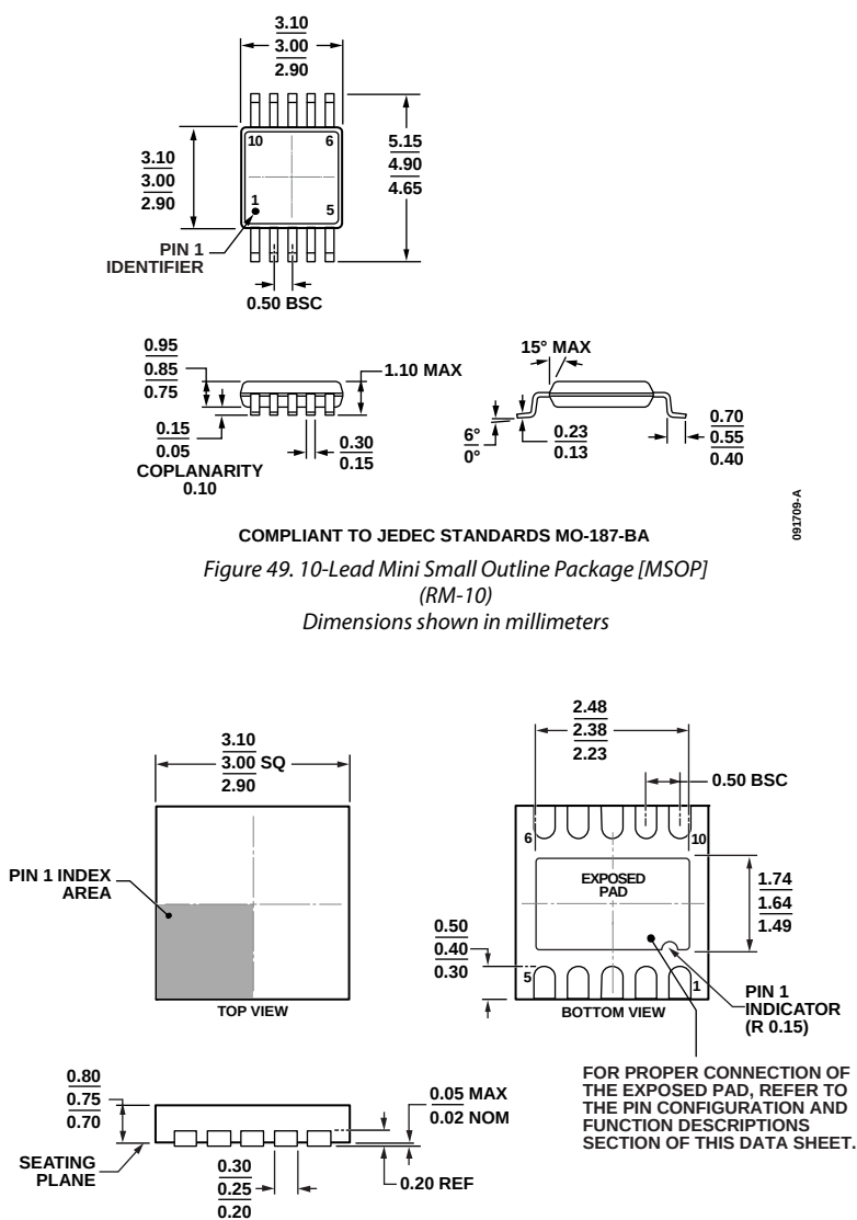
Figure 49. 10-Lead Mini Small Outline Package [MSOP] (RM-10) Dimensions shown in millimeters Figure 50. 10-Lead Lead Frame Chip Scale Package [QFN (LFCSP_WD)] 3 mm × 3 mm Body, Very Very Thin, Dual Lead (CP-10-9) Dimensions shown in millimeters
