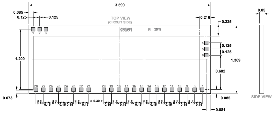
Figure 41. 28-Pad Bare Die [CHIP] (C-28-1) Dimensions shown in millimeters
