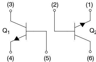
NST3904DXV6T1
