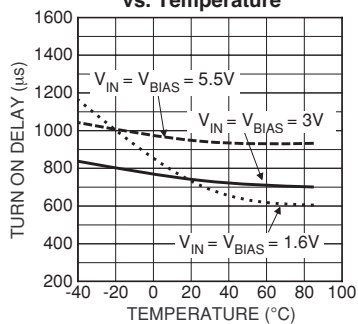
Turn On Delay vs. Temperature
