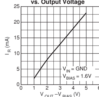
V_BIAS Reverse Current Flow vs. Output Voltage
