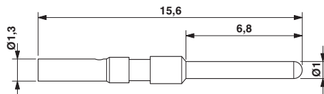
Crimp contact, diameter 1.0 mm
