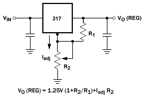
FIGURE 15. VOLTAGE REGULATOR
