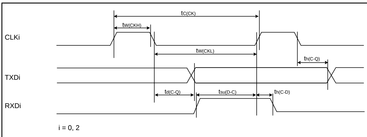
Figure 5.21 Input and Output Timing of Serial Interface
