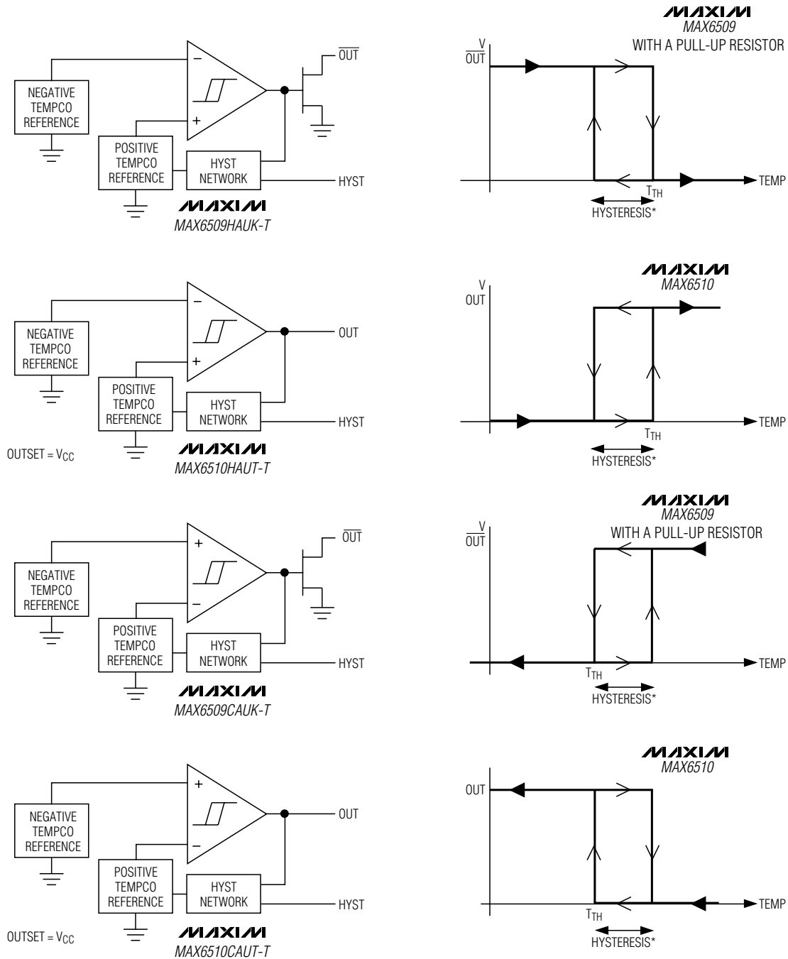
Figure 1. Block and Functional Diagrams
