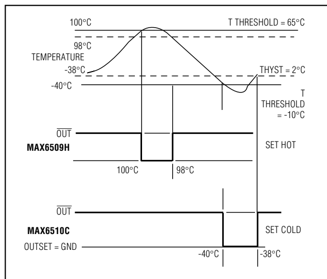
Figure 4. Temperature Response
