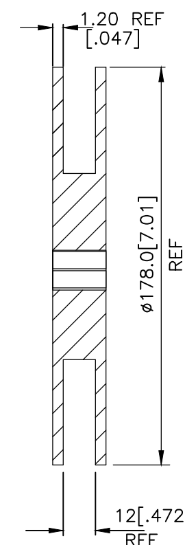
Section C—C
