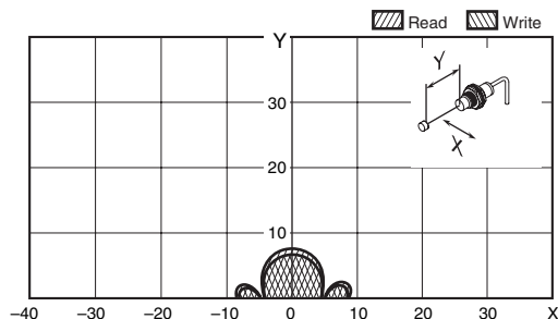
V680-HS52 (embedded in non-metallic material) & V680-D1KP53M (embedded in metallic surface: steel)
