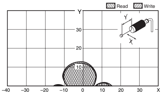
V680-HS52 (embedded in non-metallic material) & V680-D1KP53M (embedded in non-metallic material)
