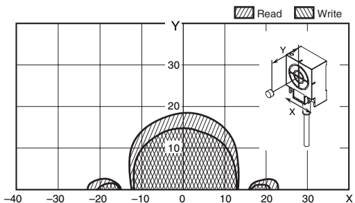
V680-HS51 (embedded in metallic material) & V680-D1KP53M (embedded in non-metallic material)
