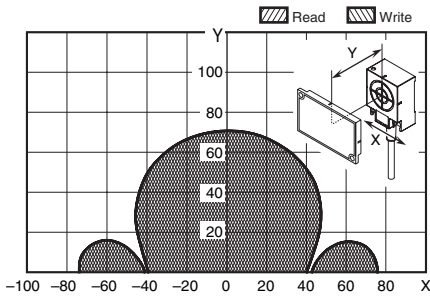
V680-HS63 (mounted on metallic material) & V680-D8KF68/-D32KF68 (mounted on metallic surface: steel) (Horizontal-facing RF Tag) V680-HS63 (mounted on metallic material) & V680-D8KF68/-D32KF68 (mounted on metallic surface: steel) (Vertical-facing RF Tag) When the V680-A81 attachment is mounted on RF Tag
