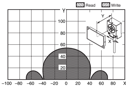
V680-HS65 (mounted on metallic material) & V680-D8KF68/-D32KF68 (Horizontal-facing RF Tag) V680-HS65 (mounted on metallic material) & V680-D8KF68/-D32KF68 (Vertical-facing RF Tag)
