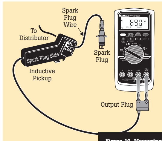
Figure 14. Measuring RPM with the RPM80 Inductive Pickup
