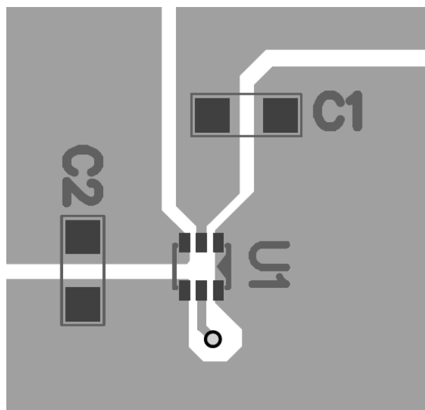
Figure 2: Recommended Layout
