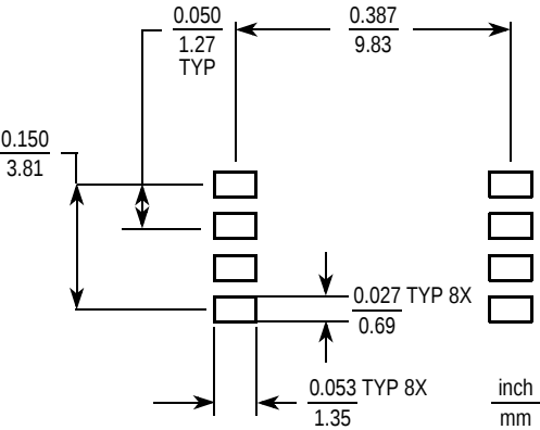
Figure 9. SSOP footprint
