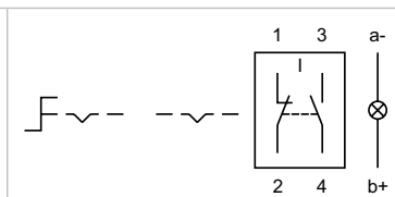
Wiring diagram 23
