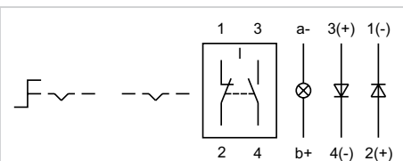
Wiring diagram 21
