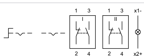
Wiring diagram 26
