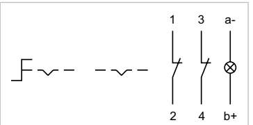
Wiring diagram 18
