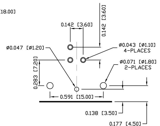
PCB LAYOUT
