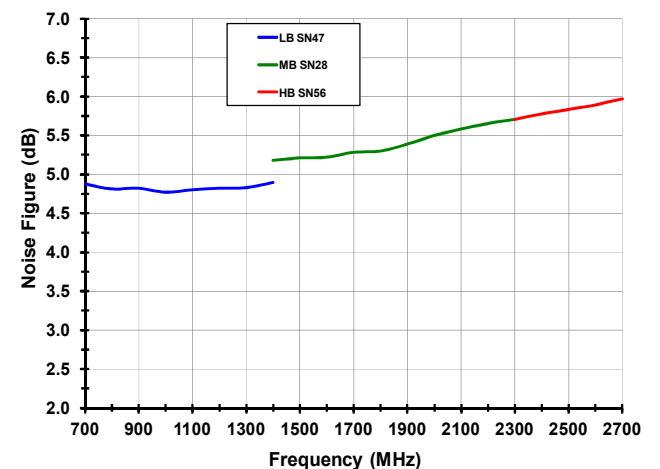
Worst Case NF vs. Frequency [105C, 5.25V]
