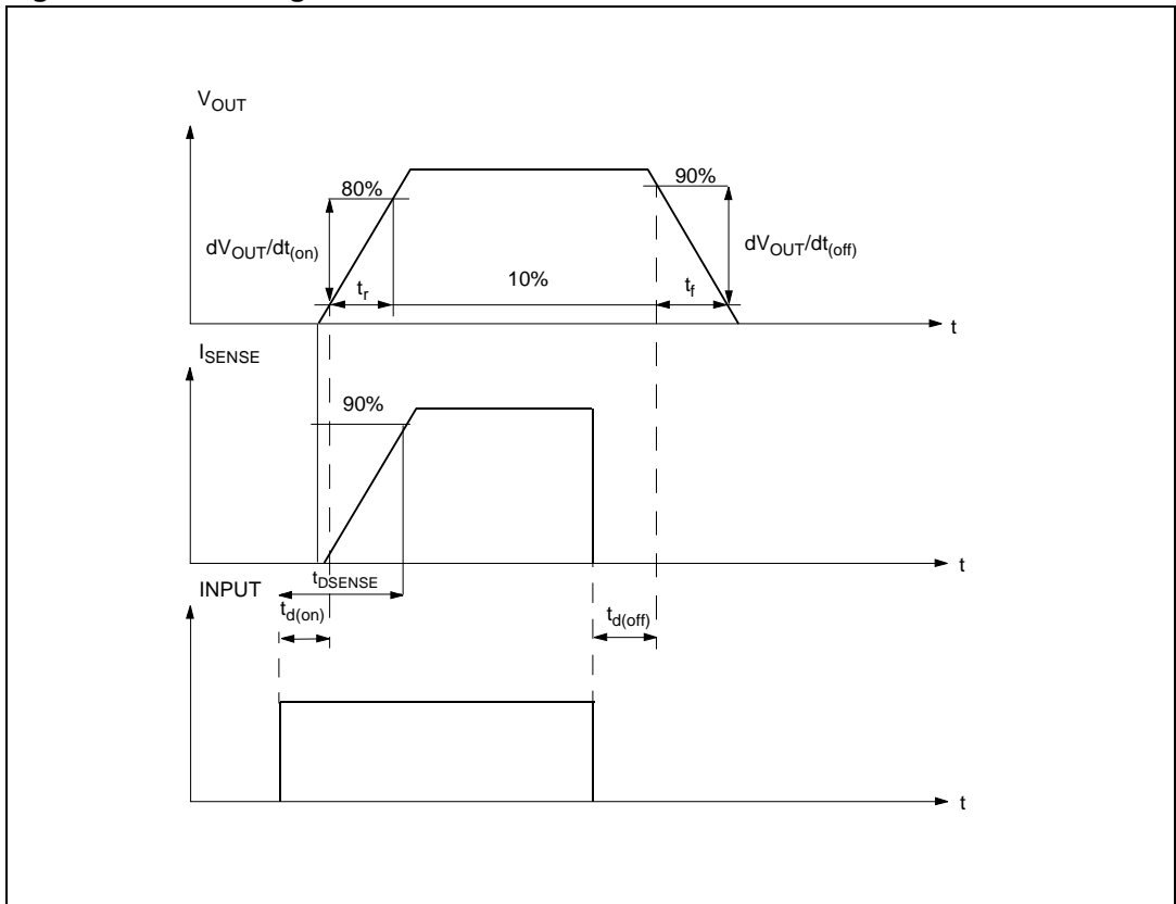
Figure 5. Switching characteristics
