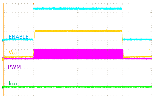
Start-up/Shutdown, ENABLE At No Load, 10 ms/div
