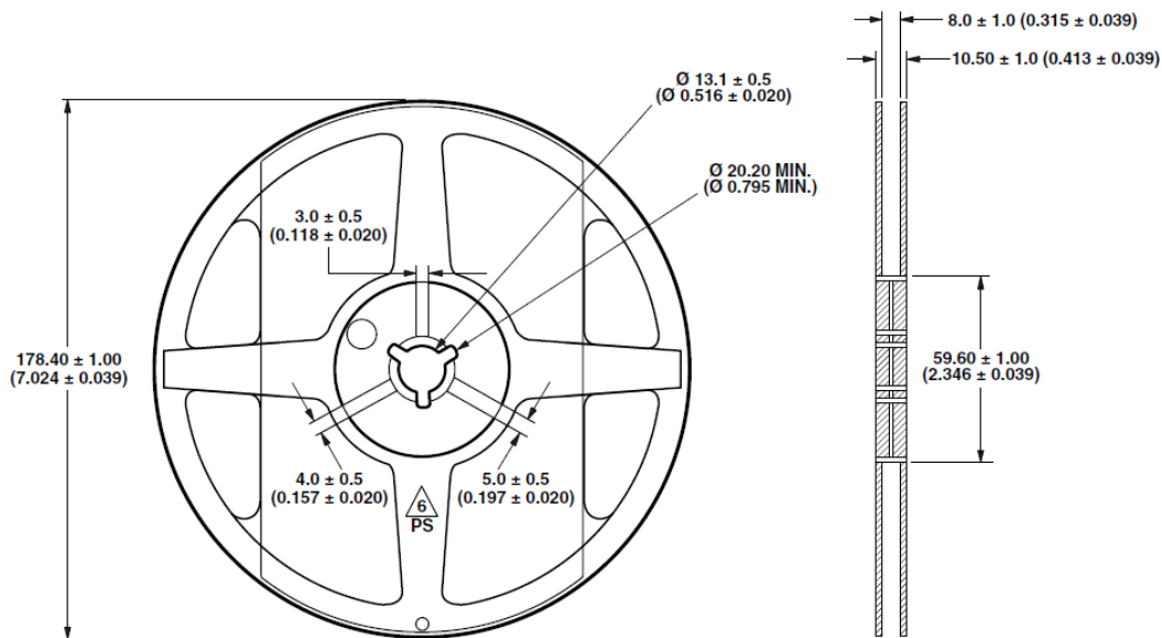
Figure 12: Reel Dimensions
