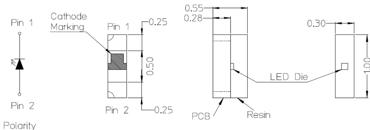
Figure 1: Package Dimensions
