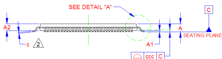
Figure 16.1 LAN9311 128-VTQFP Package Definition
