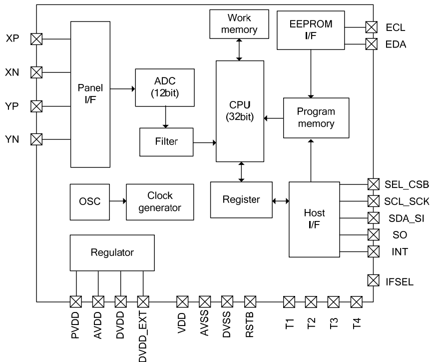
Figure 4. Block Diagram
