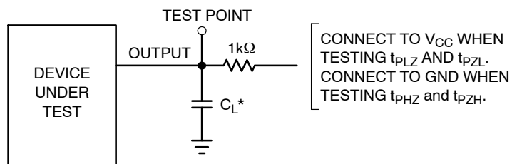
Figure 6. Test Circuit
