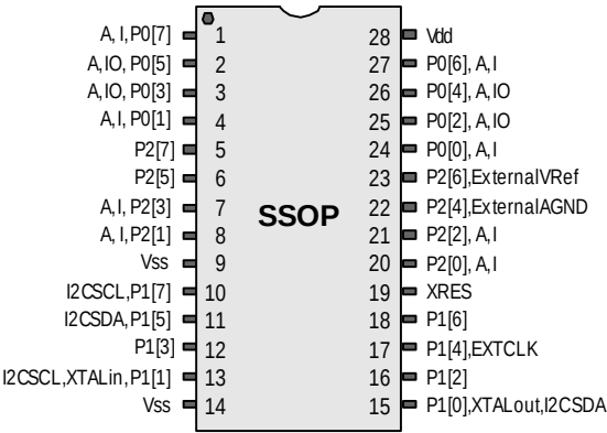
CY8C27443 28-Pin PSoC Device
