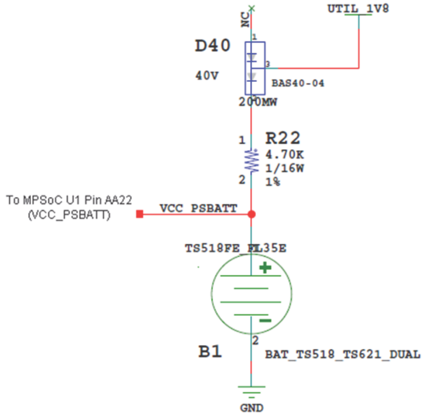
Figure 3-2: Encryption Key Backup Circuit
