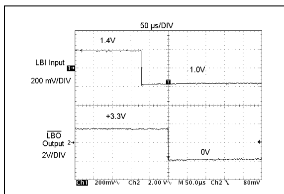
FIGURE 2-24: LBO Output Timing.
