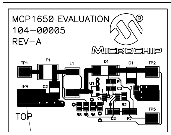
FIGURE 6-2: Top Layer Wiring.
