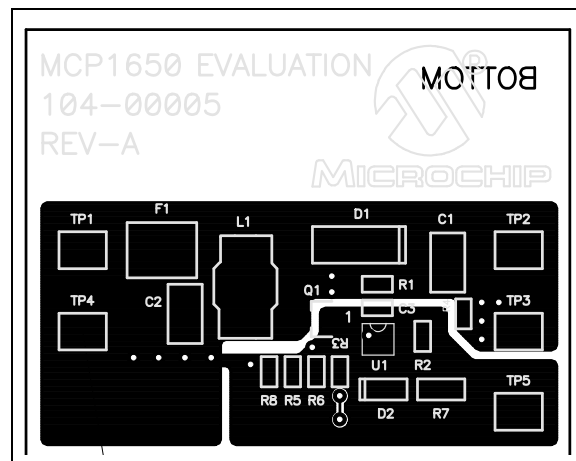
FIGURE 6-3: Bottom Layer Wiring.
