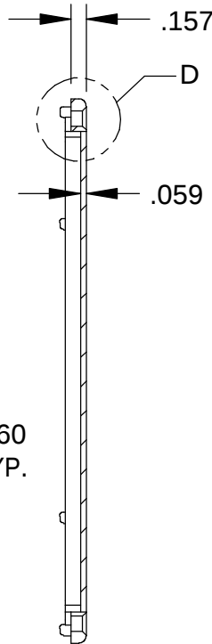
SECTION C-C
