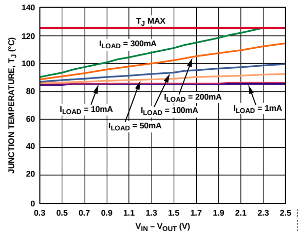
Figure 36. T_A = 85^\circ\text{C}
