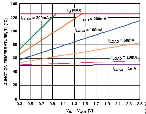
Figure 35. 0 mm² of PCB Copper, T_A = 50^\circ\text{C}
