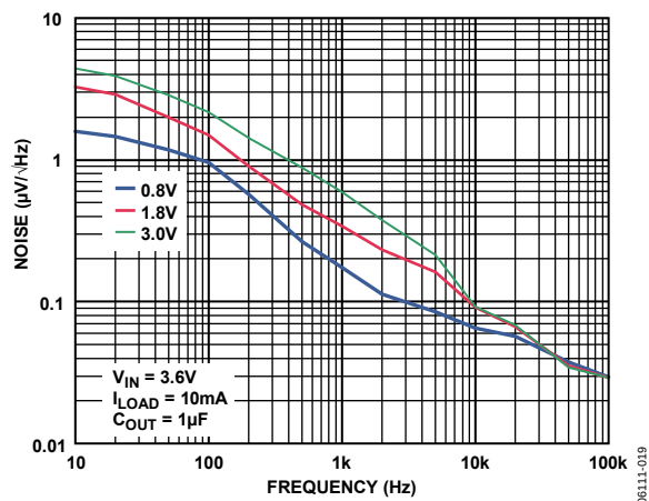
Figure 17. Output Noise Spectrum
