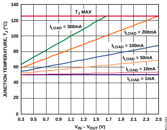
Figure 33. 500 mm² of PCB Copper, T_A = 50^\circ\text{C}
