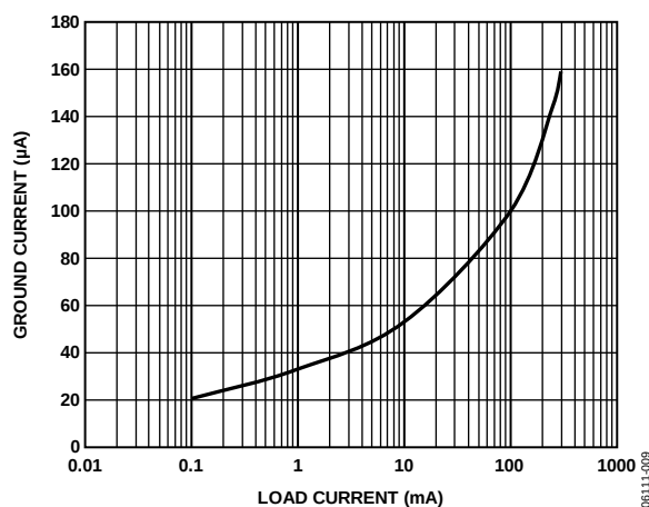
Figure 7. Ground Current vs. Load Current
