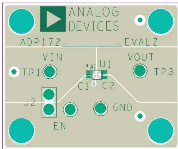
Figure 37. Example ADP172 PCB Layout
