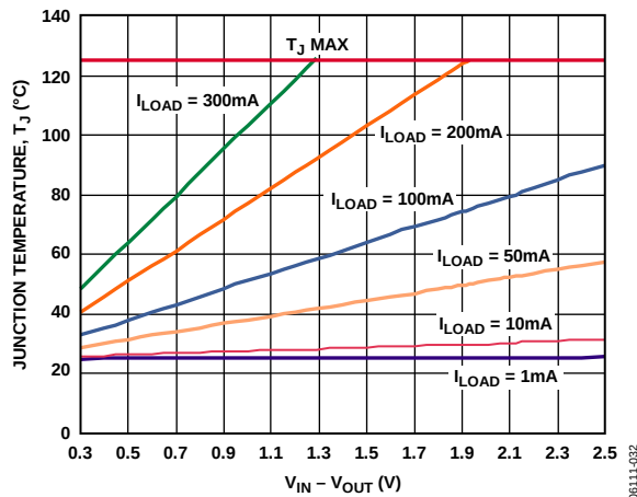
Figure 32. 0 mm² of PCB Copper, T_A = 25^\circ\text{C}
