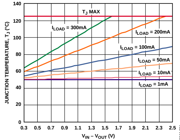
Figure 34. 100 mm² of PCB Copper, T_A = 50^\circ\text{C}
