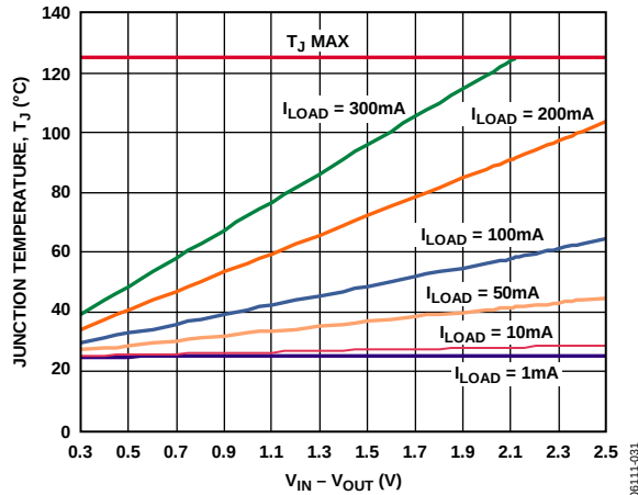
Figure 31. 100 mm² of PCB Copper, T_A = 25^\circ\text{C}
