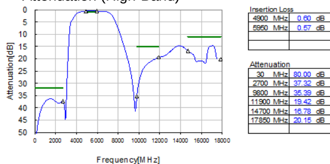
Attenuation (High-Band)
