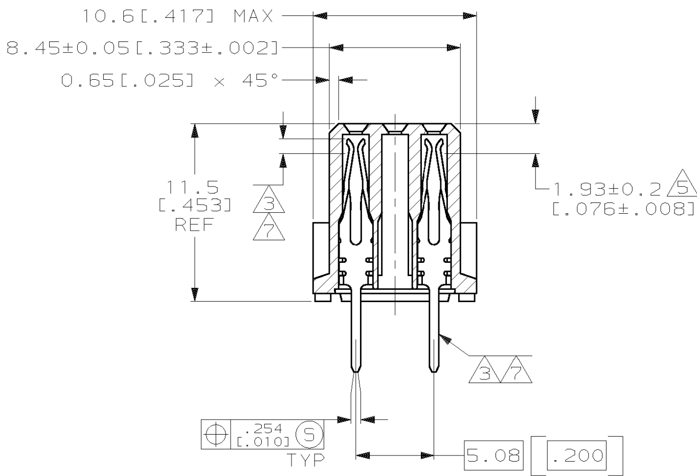
SECTION X-X
