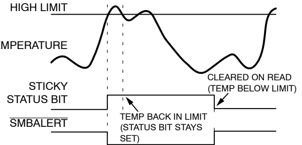
Figure 38. ALERT and Status Bit Behavior
