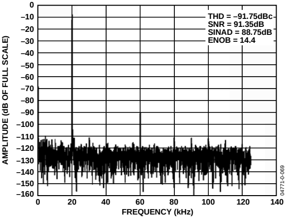
Figure 71. AD8137 Performance on +6 V, -1 V Supplies, -0.45 dBFS
