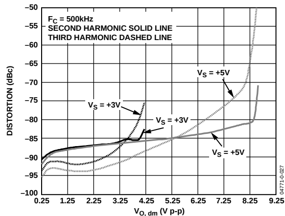
Figure 19. Harmonic Distortion vs. Output Amplitude and Supply, F_C = 500 kHz
