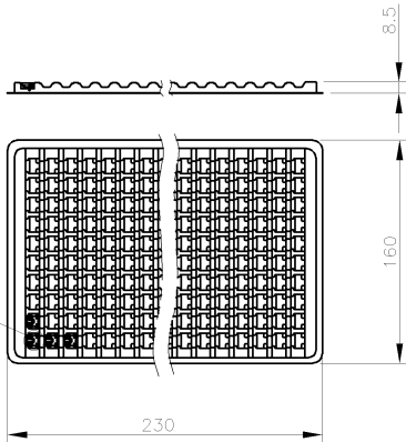
TRAY LAYOUT
