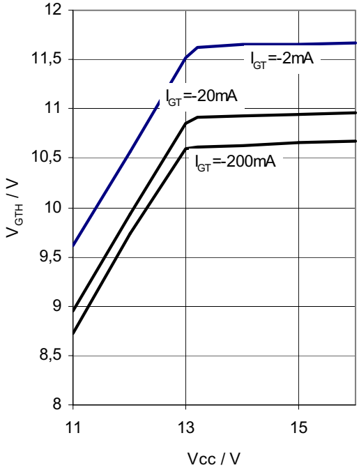
Gate Drive Voltage High State versus V CC
