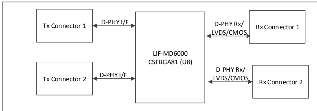
Figure 3.2. Bridging Block
