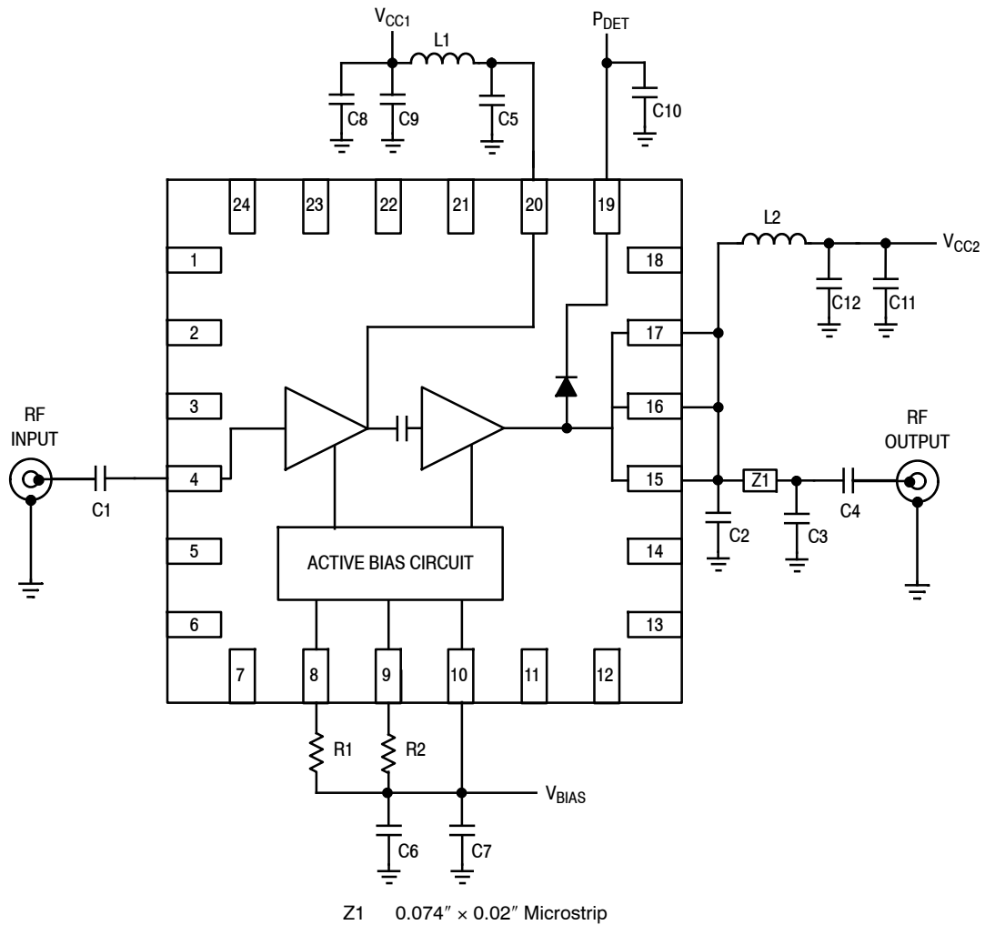
Figure 3. MMZ25332B4T1 Test Circuit Schematic
