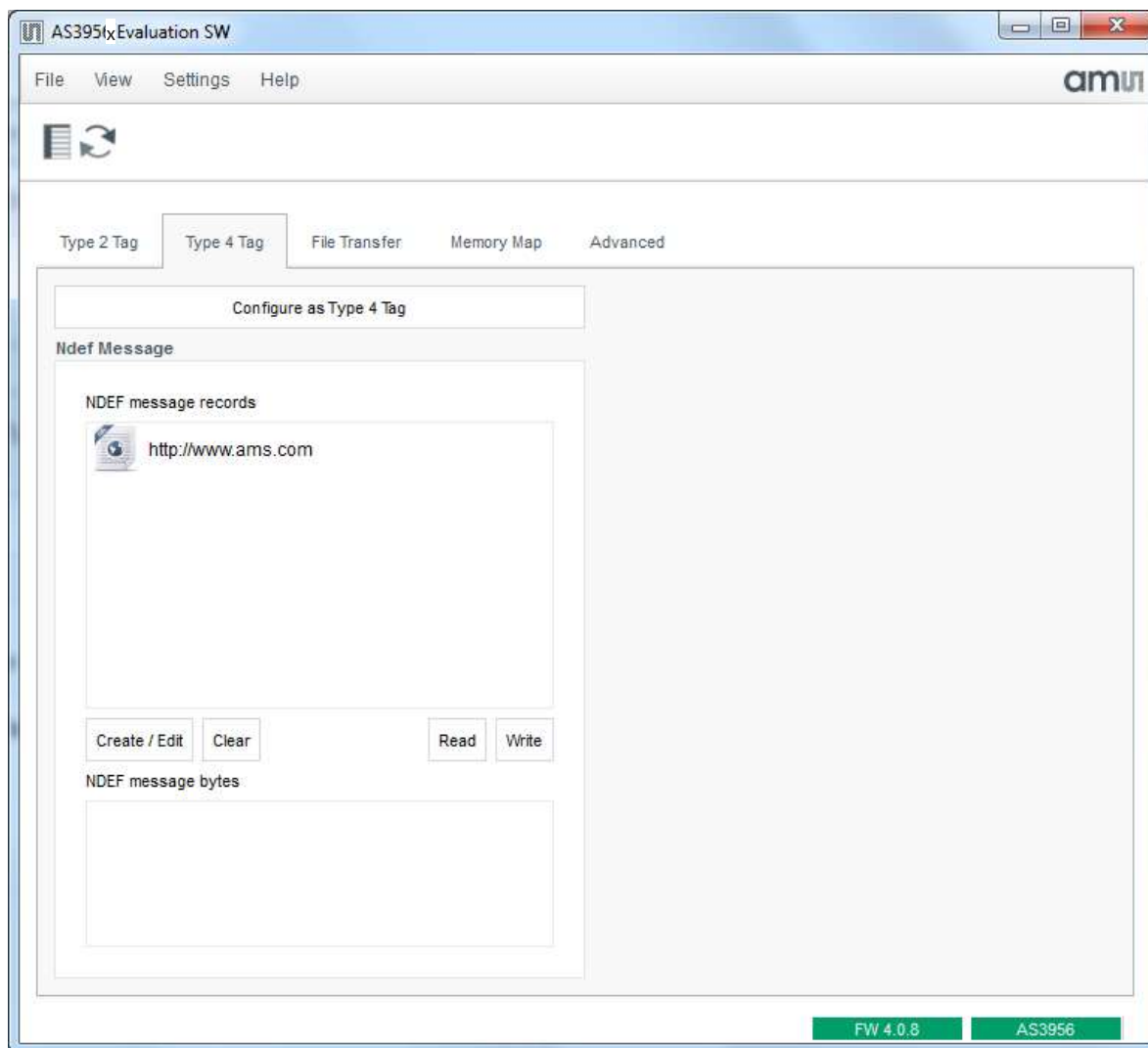
Figure 10: AS3956 GUI – Type 4 Tag tab
