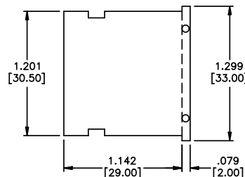
DPS910A2 Spacer
