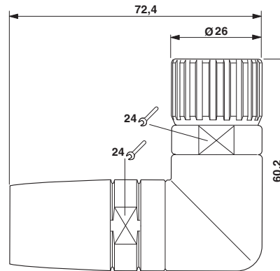
Dimensional drawing
