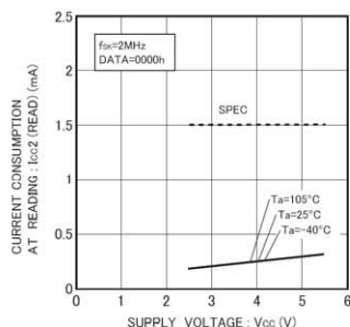
Fig.41 Consumption current at READ action I_{CC2}(READ, f_{SK}=2MHz)
