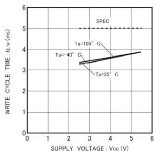
Fig.56 Write cycle time tEW
