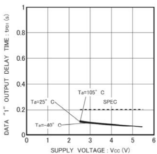
Fig.53 Output data "1" delay time tPD1
