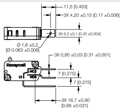
Figure 10. V15 Series M-style Short Solder Terminal
