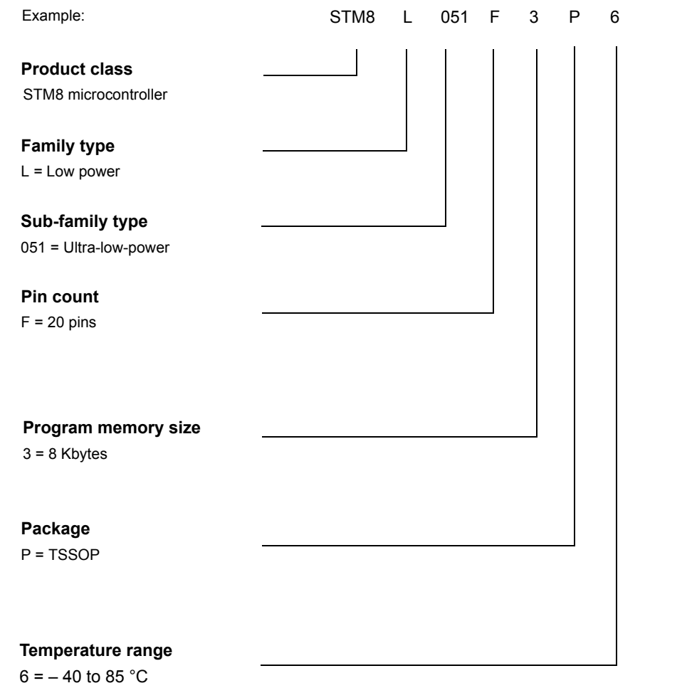
Figure 41. Low density value line STM8L051F3 ordering information scheme
