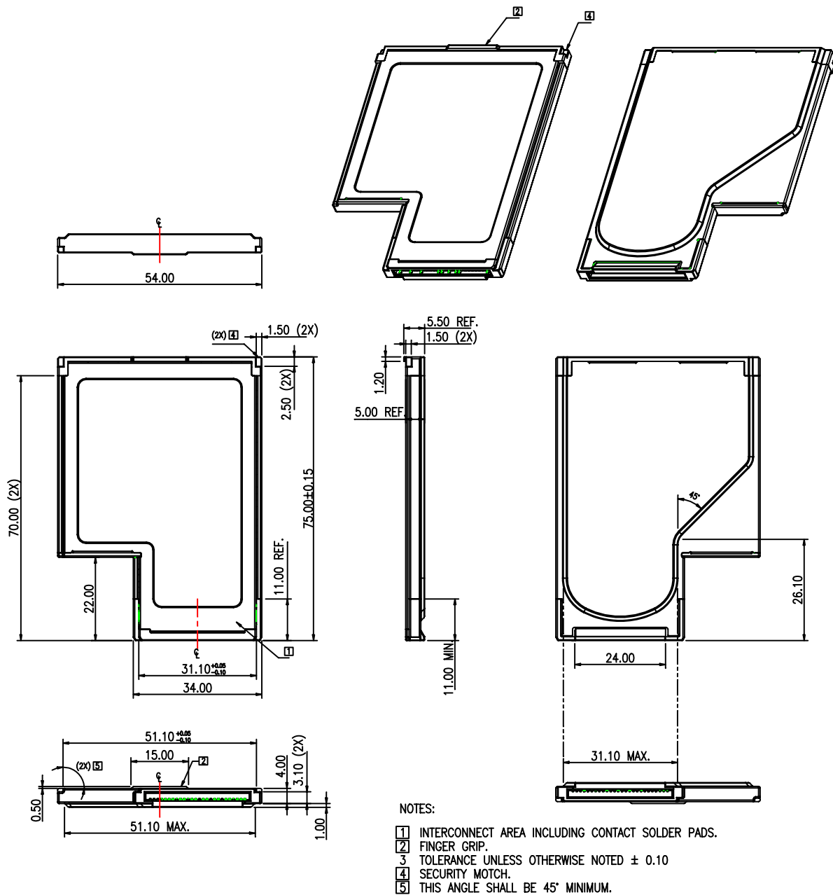
Figure: ExpressCard/34 Module Outline Dimensions
