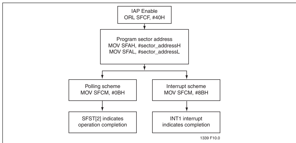
Figure 11: Sector-Erase
