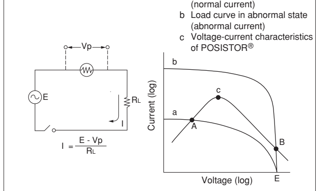
Load Curve of Circuit and Voltage - Current Characteristics of POSISTOR®
