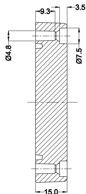
SECTION B-B
